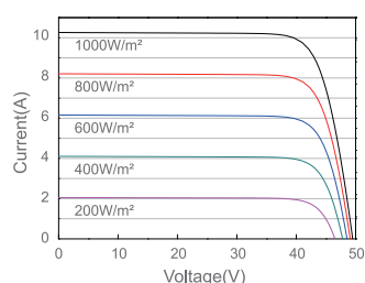
Current-Voltage Curve JAM72S10-400/PR
