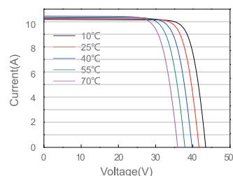
Current-Voltage Curve JAM60D10-340/MB
