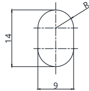
Mounting Hole
