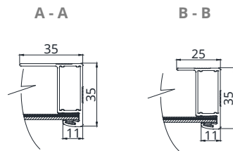
Frame Cross Section
